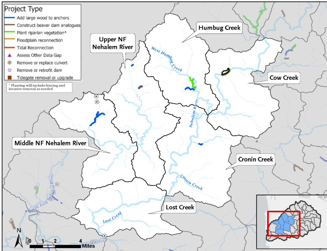
Figure 6-4 Near-term Projects Proposed in the Middle and Upper North Fork Nehalem and Humbug Creek Focal Areas, and Neighboring Cow, Cronin, and Lost Creek Subwatersheds.
