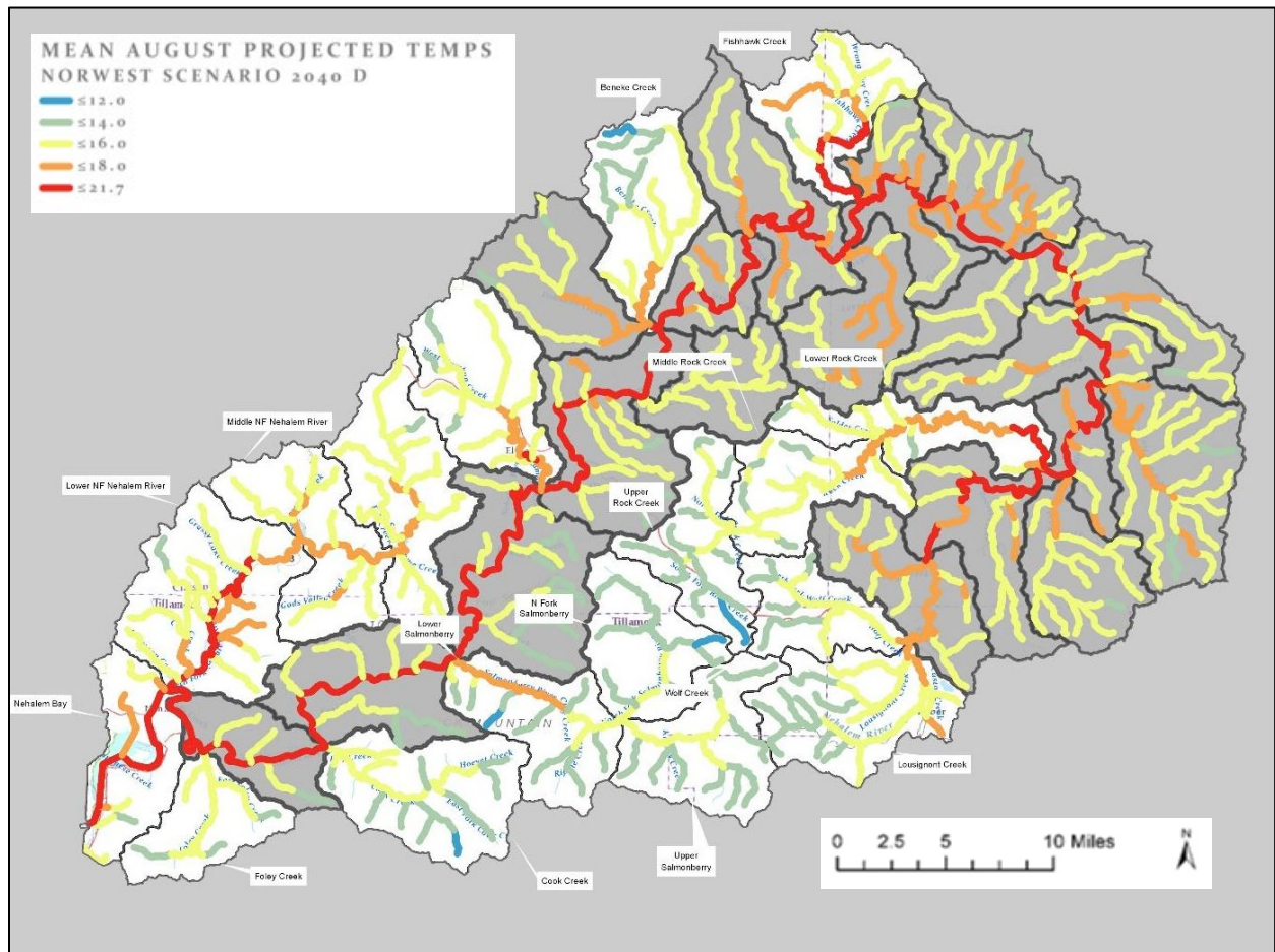
Figure 5-7 Modeled 2040 Stream Temperatures in the Nehalem River Watershed.
